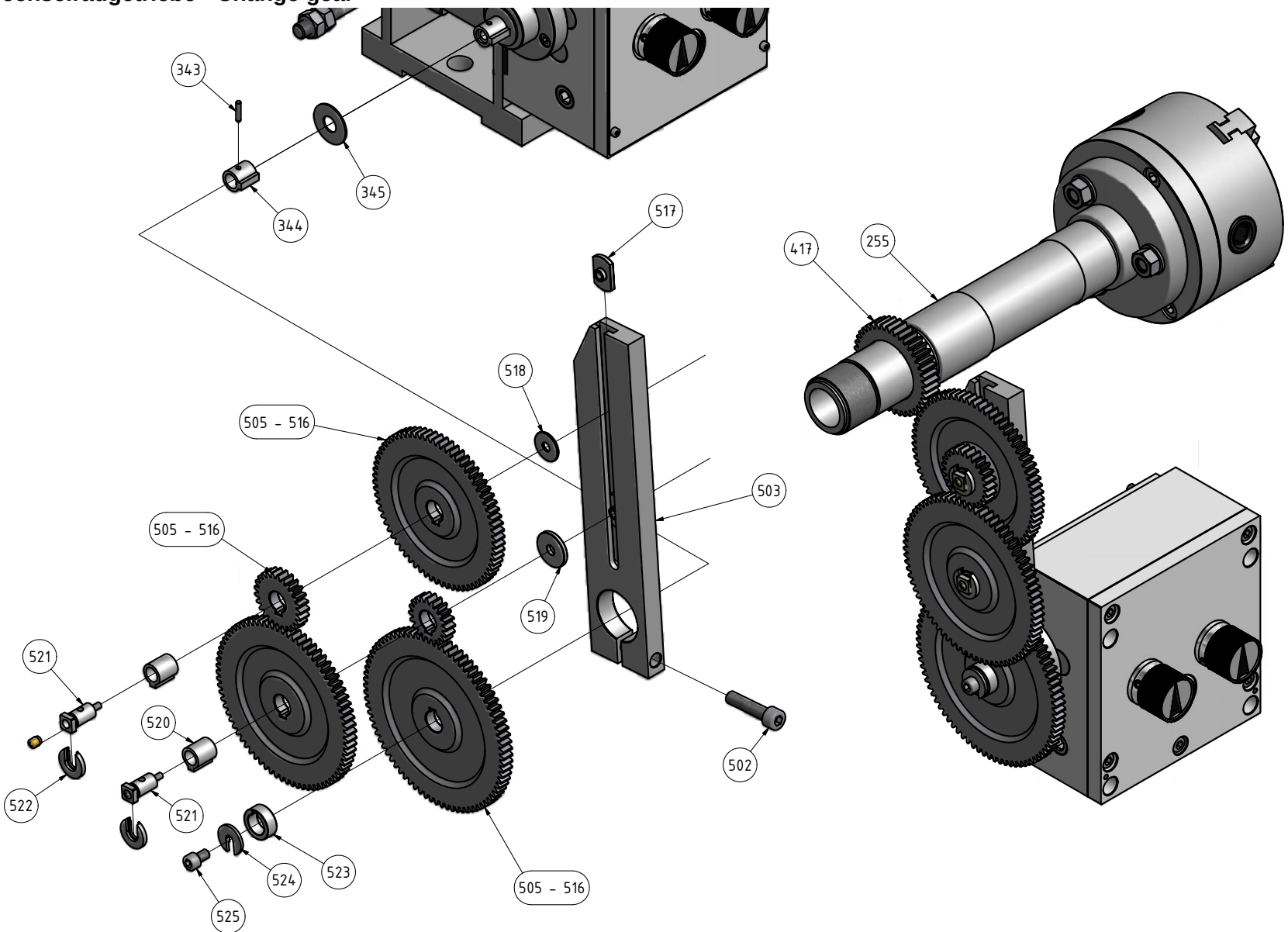
1-11: Change gear
