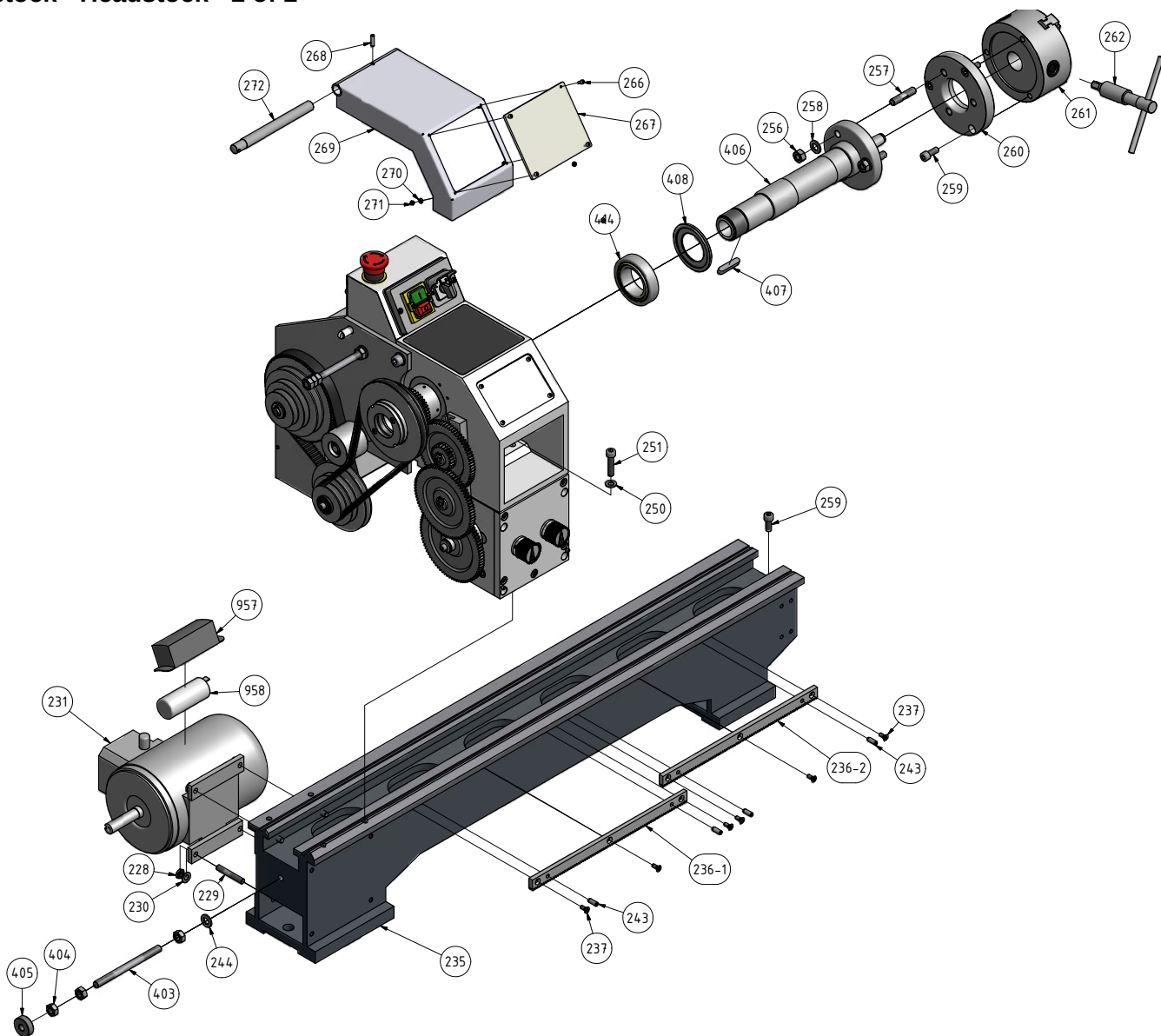
1-10: Headstock D240 2 of 2
