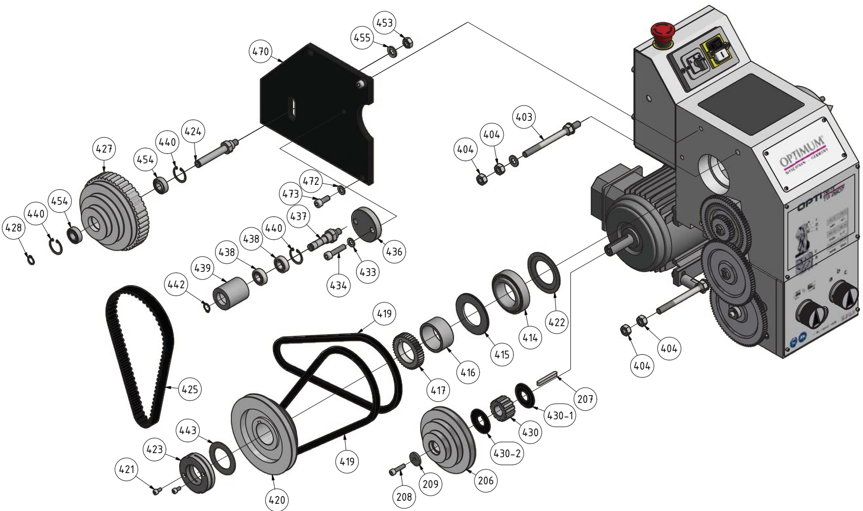
2-9: Headstock
