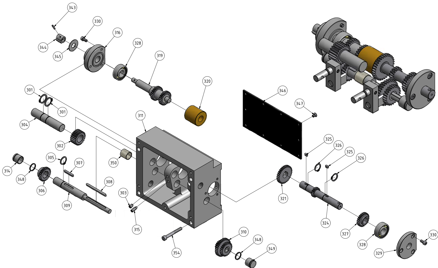
2-8: Feed gear D280 2 of 2
