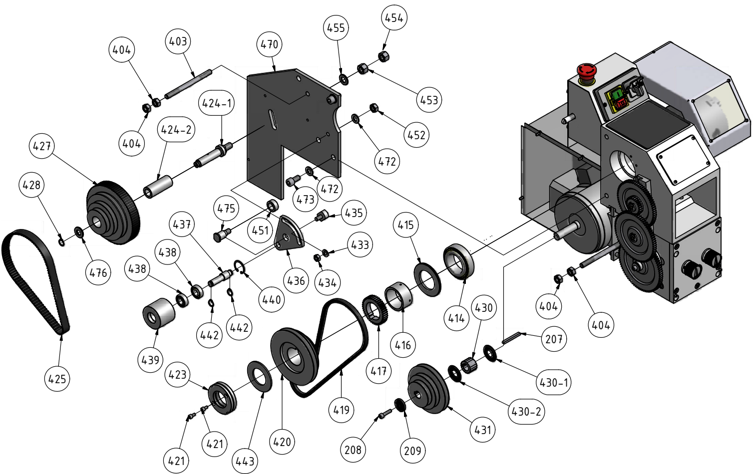
1-9: Headstock D240 1 of 2
