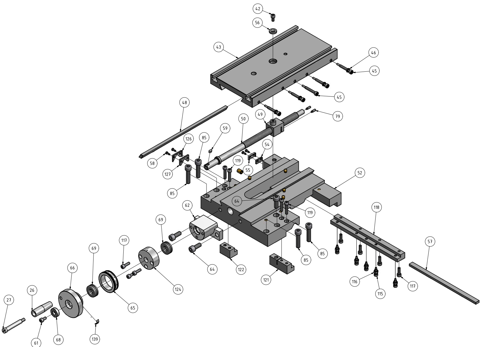
1-2: Cross slide D240
