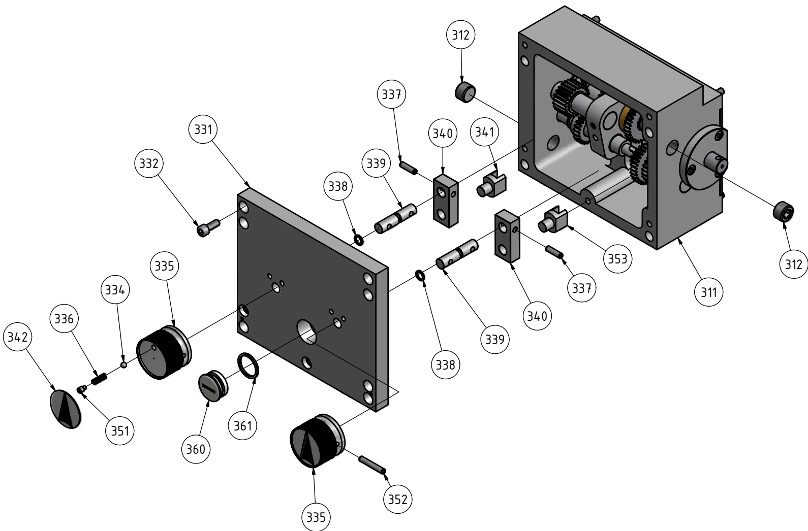
2-7: Feed gear D280 1 of 2
