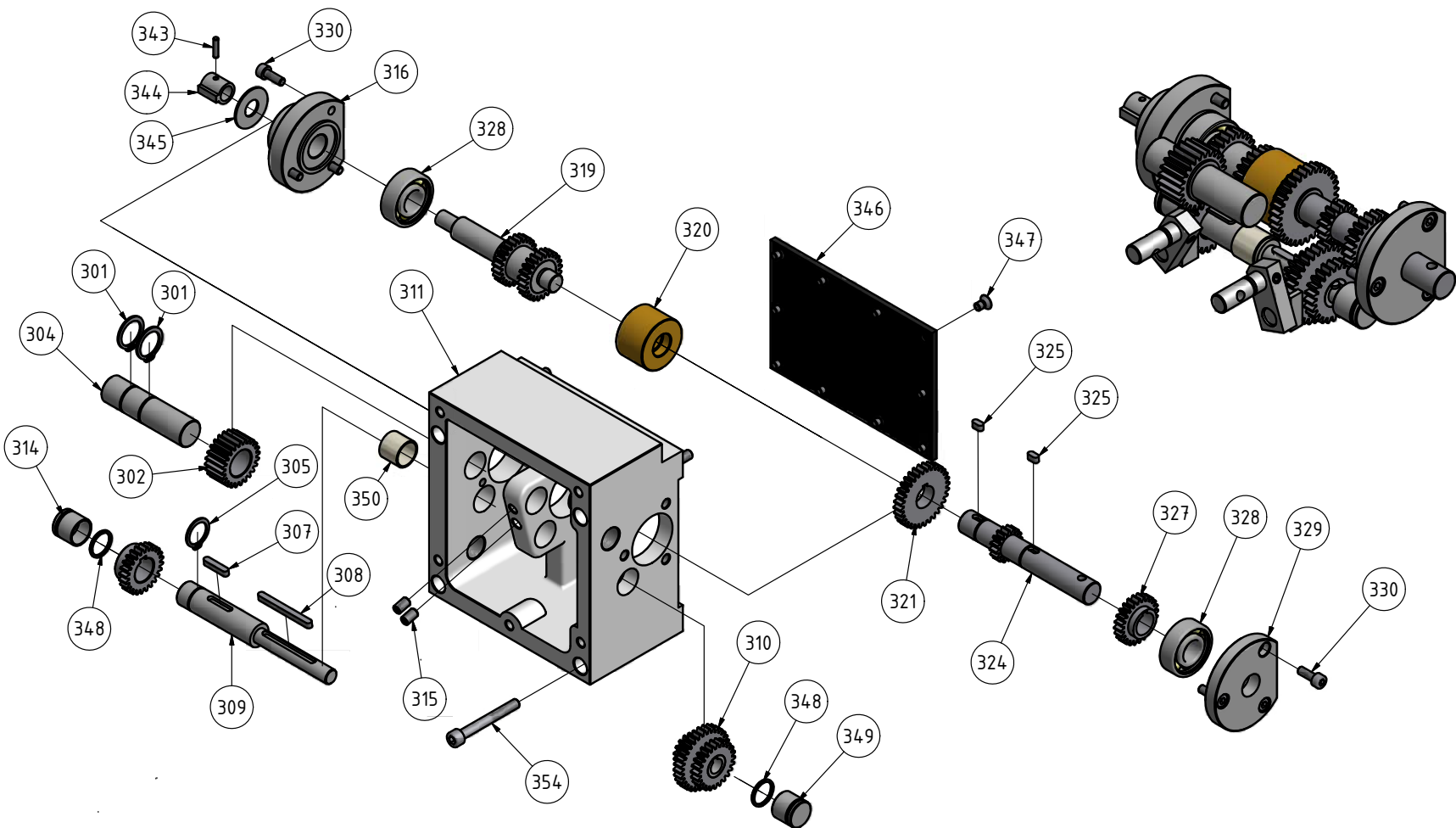
1-8: Feed gear D240 2 of 2
