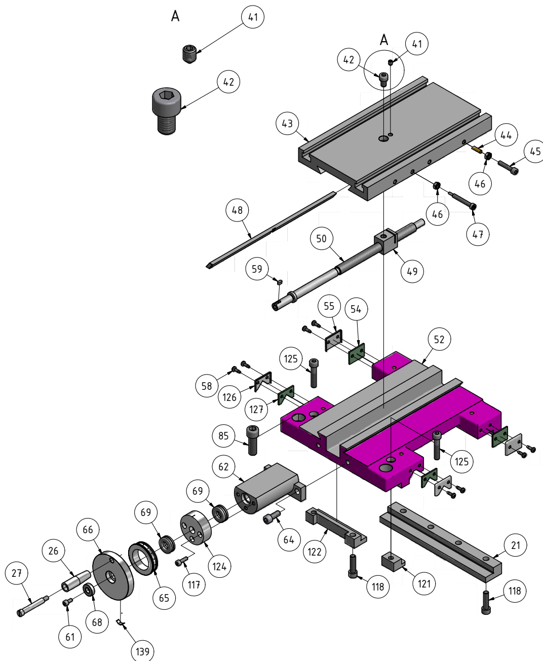
2-2: Cross slide
