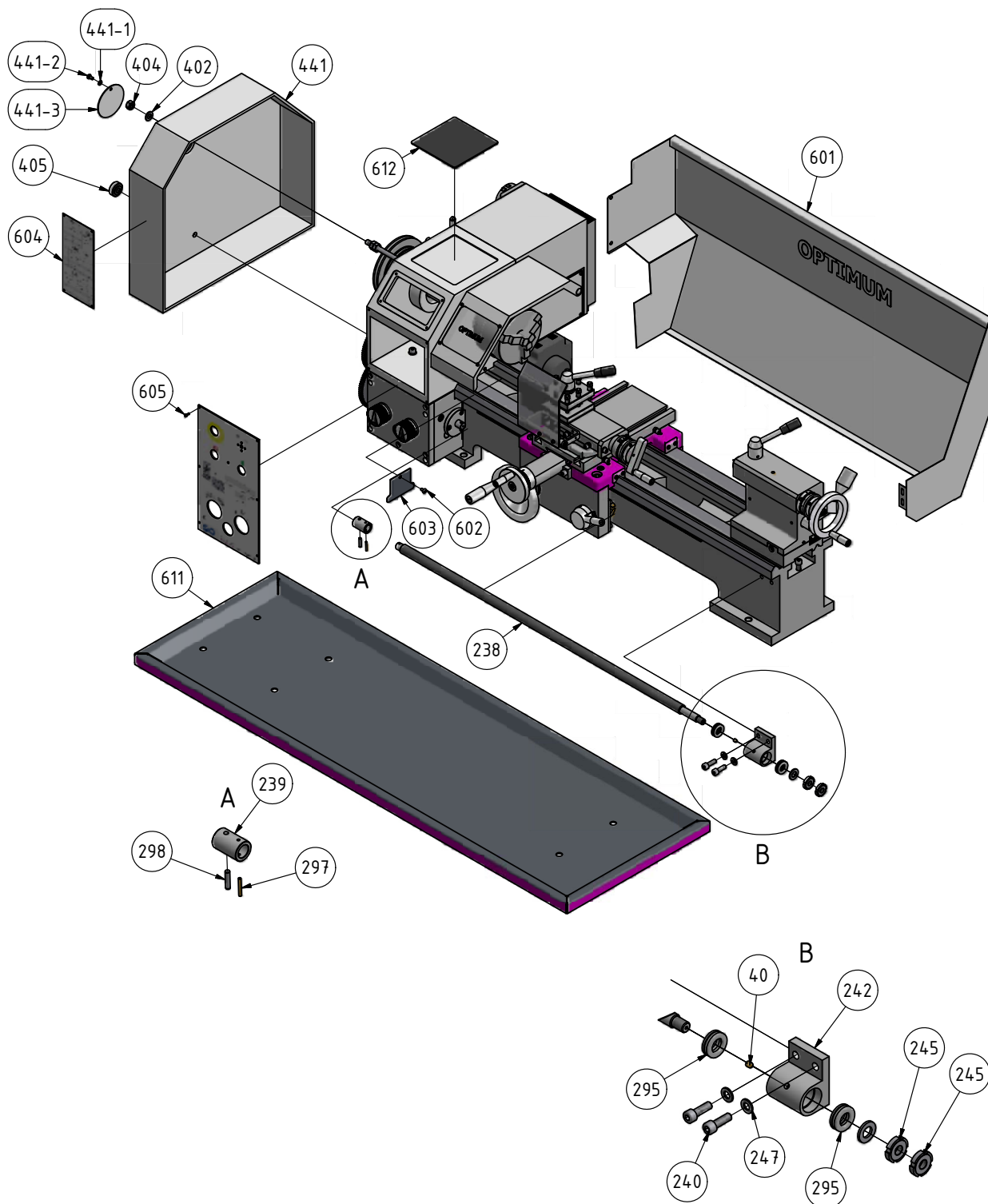
2-6: Machine bed
