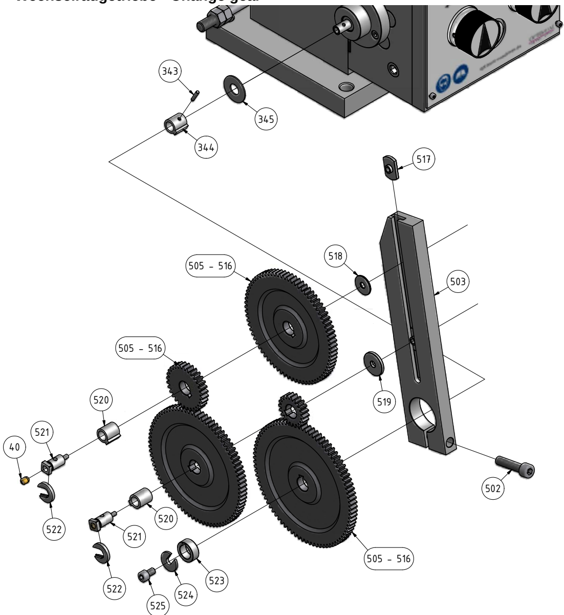
2-10: Change gear
