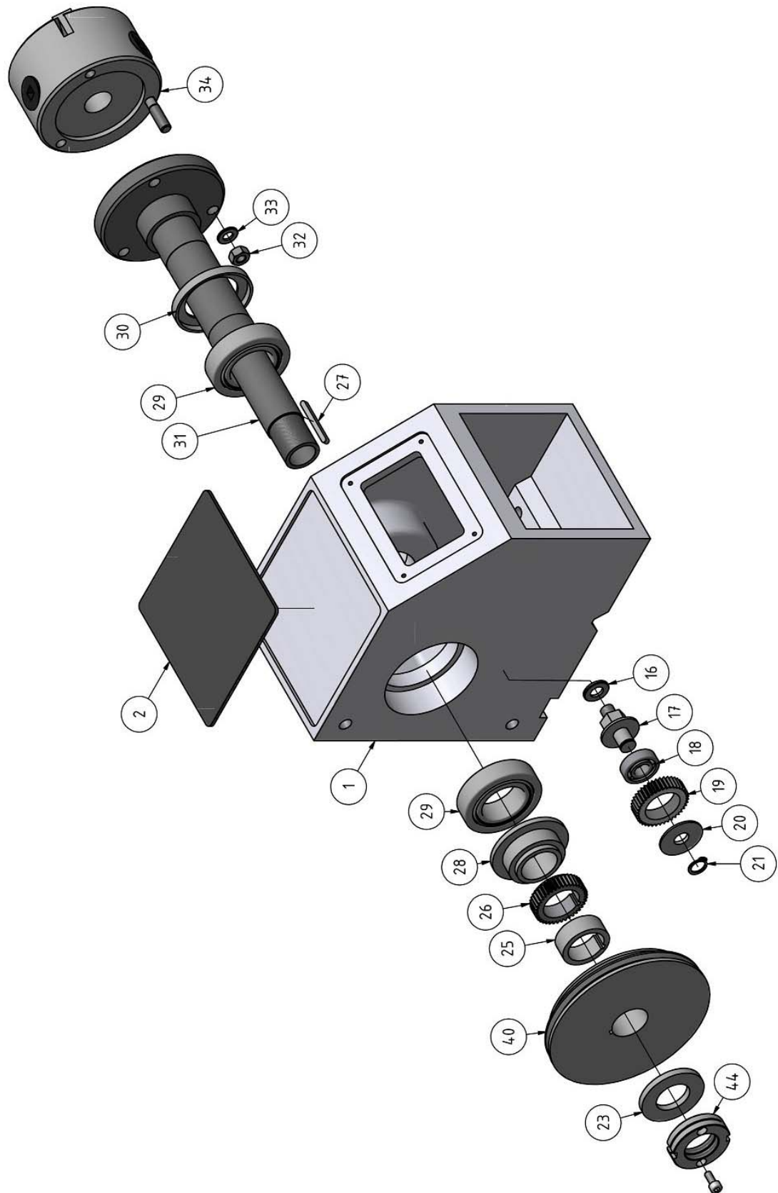
Abb.6-7: Spindelstock - Headstock
