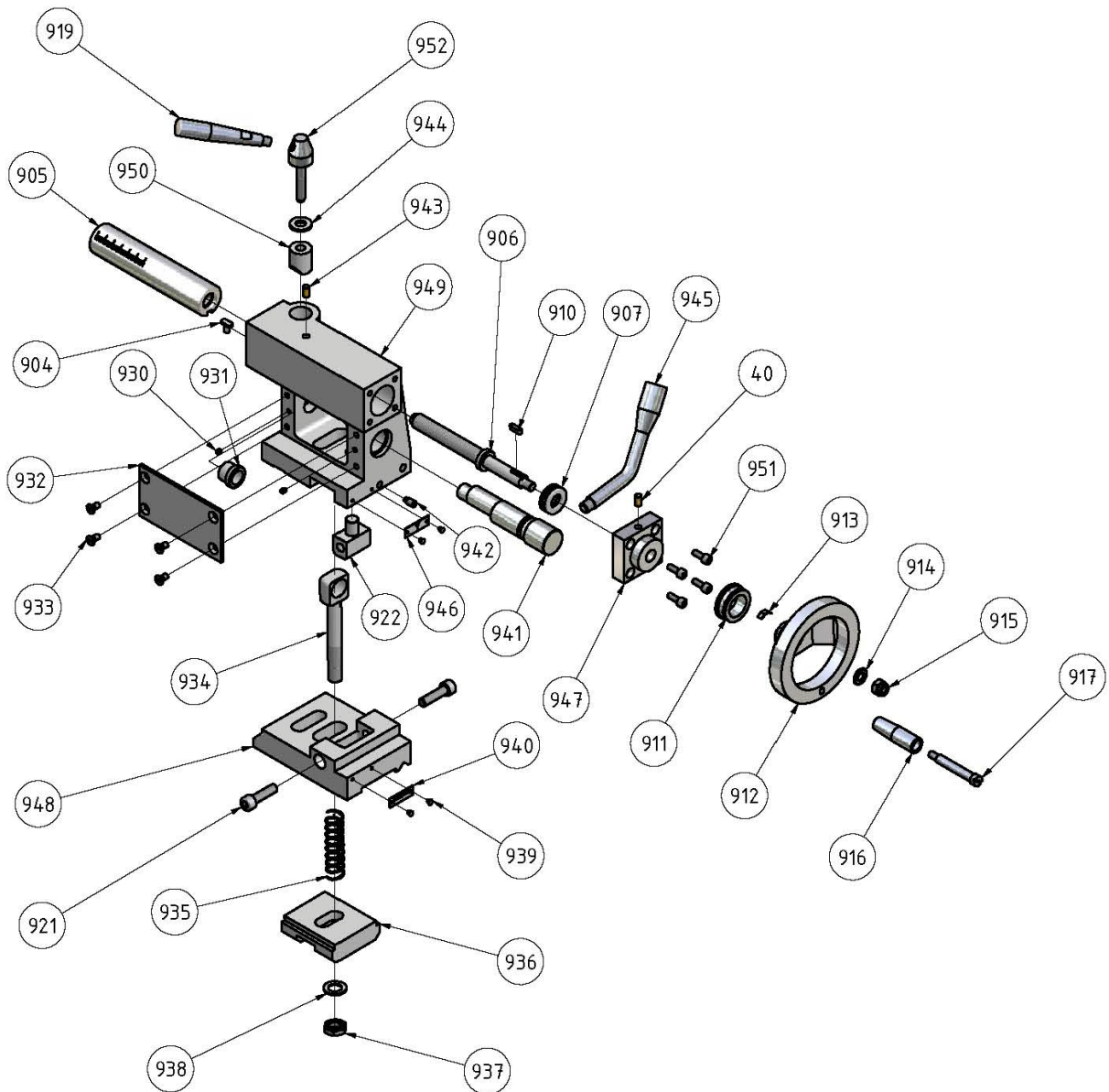
Abb.6-5: Reitstock - Tailstock
