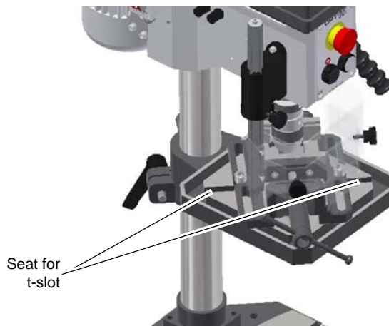
Abb. 1-2: Drilling table
