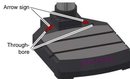
Abb.3-1: Marking of fixing points on bench drills
