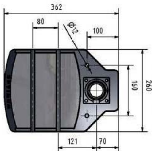
Abb.3-2: B16H
