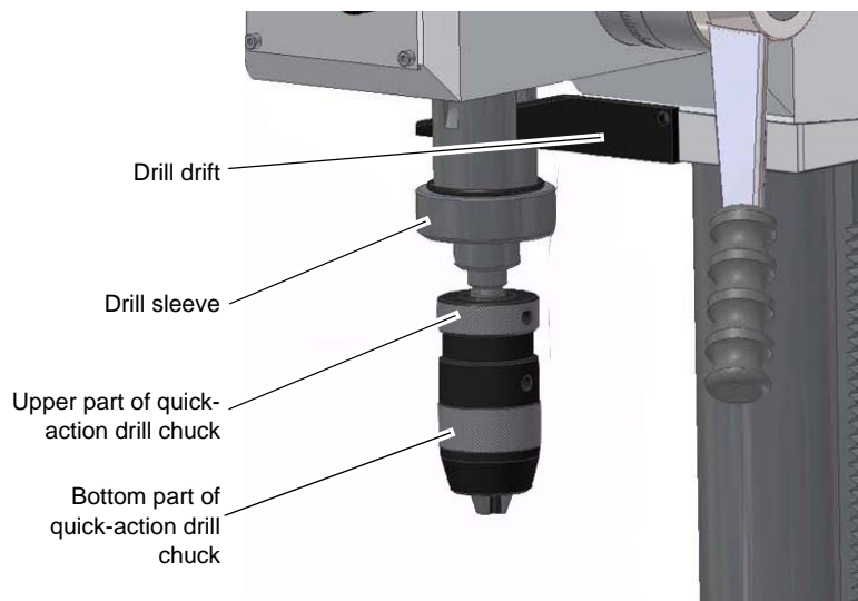
Abb.4-7: Unfitting the drill chuck
