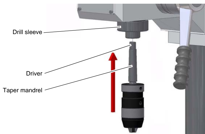
Abb. 4-5: Taper mandrel
