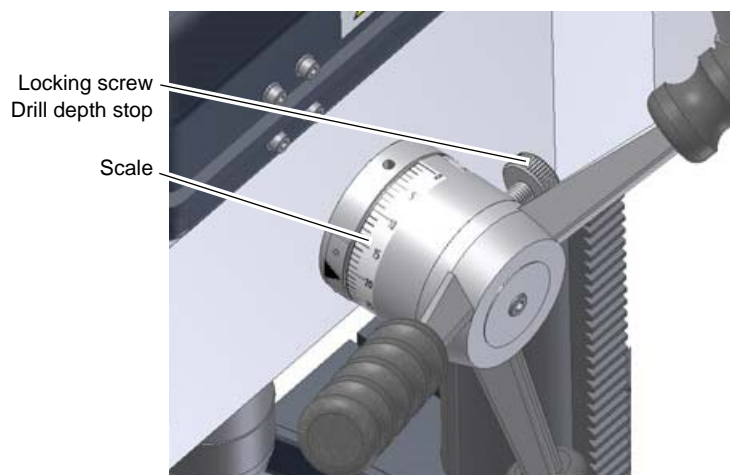
Abb.4-3: Drill depth stop
