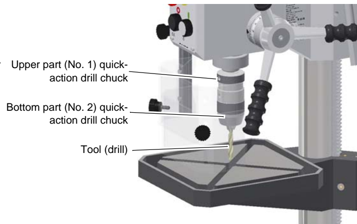
Abb.4-6: Quick-action drill chuck
