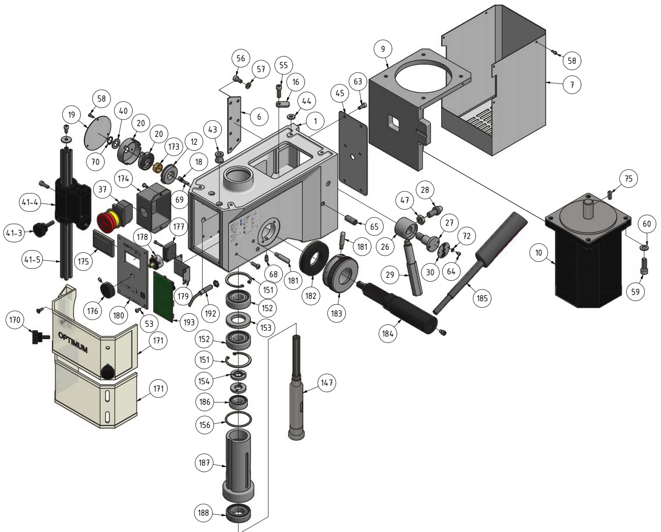
Abb.1-1: Bohrkopf - Drilling head
