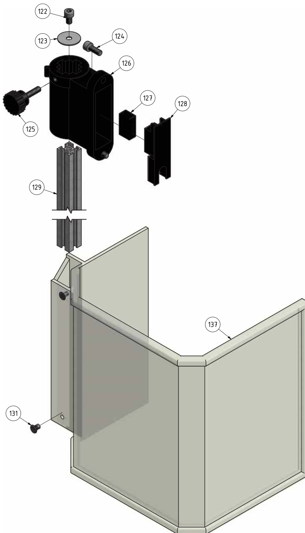
Abb.1-17: Bohrfutterschutz - Drilling chuck protection
