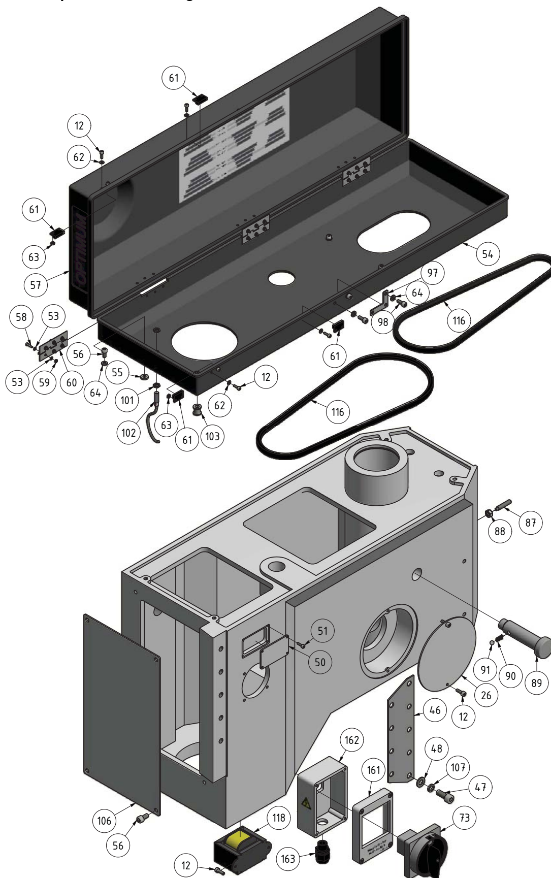
Abb.1-6: Bohrkopf 5 von 5 - Drilling head 5 of 5
