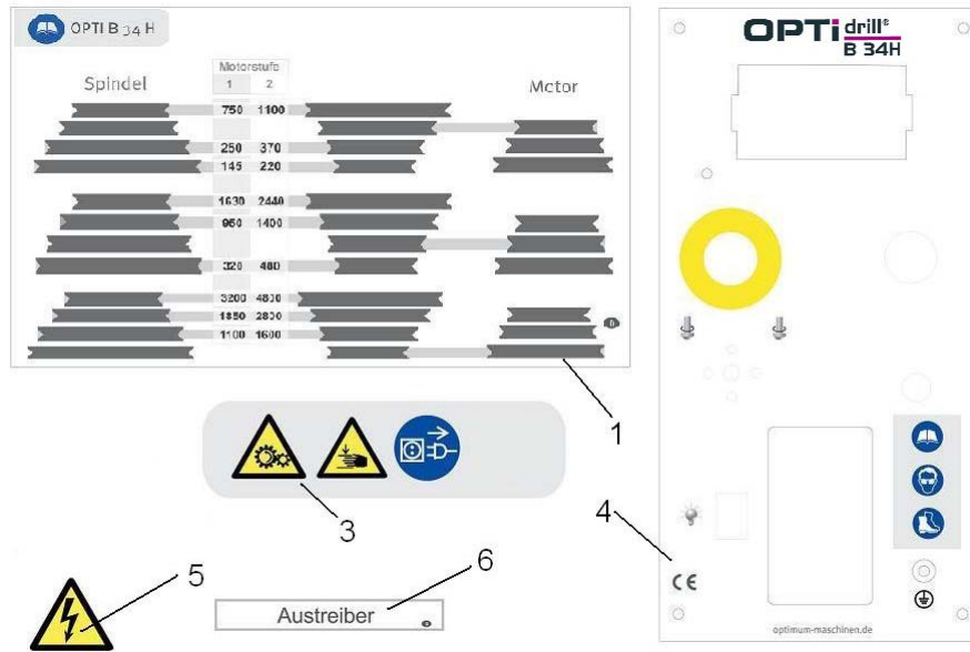
Abb.1-9: Maschinenschilder - Machine labels B34H
