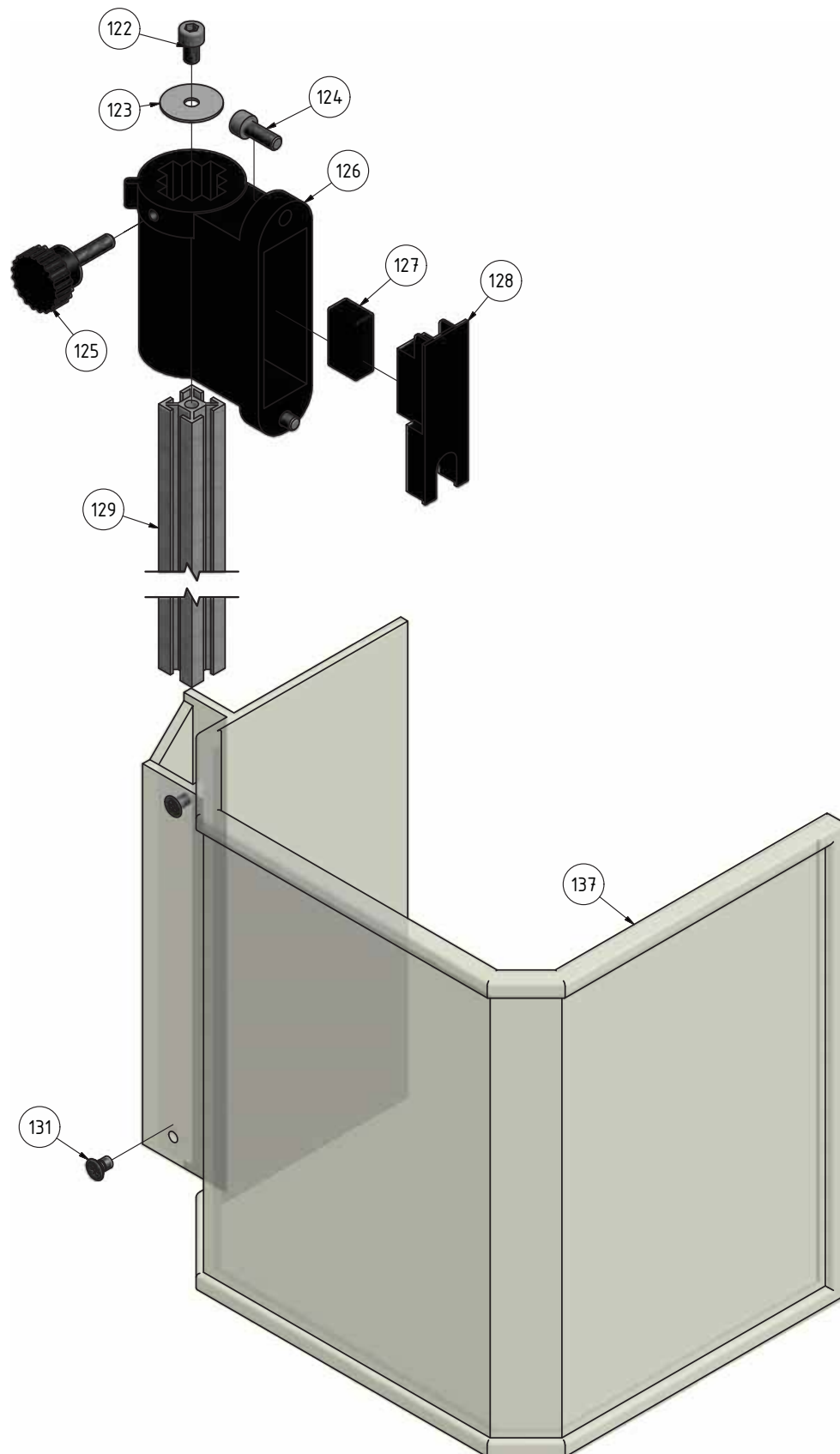
Abb.1-7: Bohrfutterschutz - Drilling chuck protection
