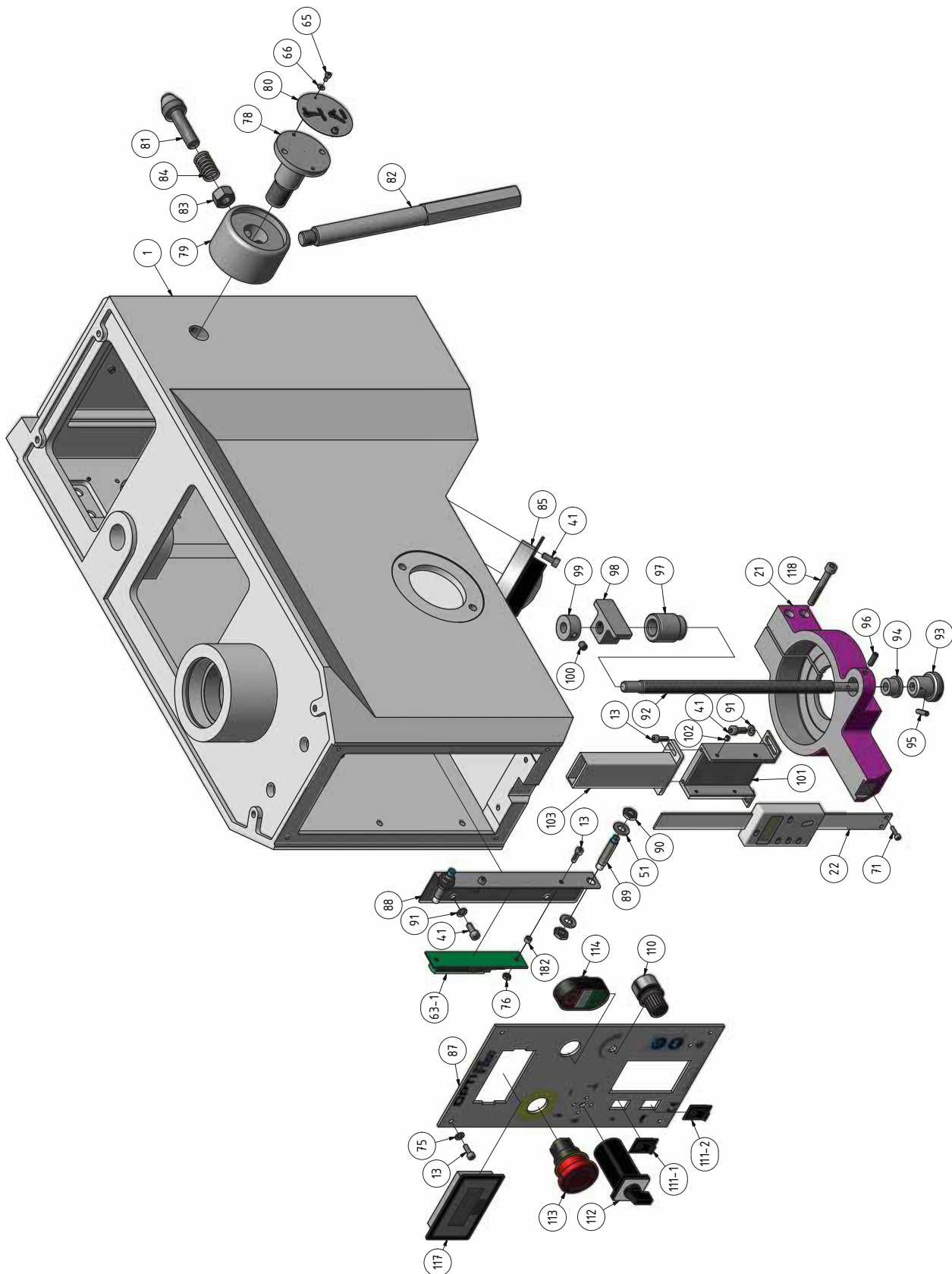
Abb.1-15: Bohrkopf 4 von 5 - Drilling head 4 of 5
