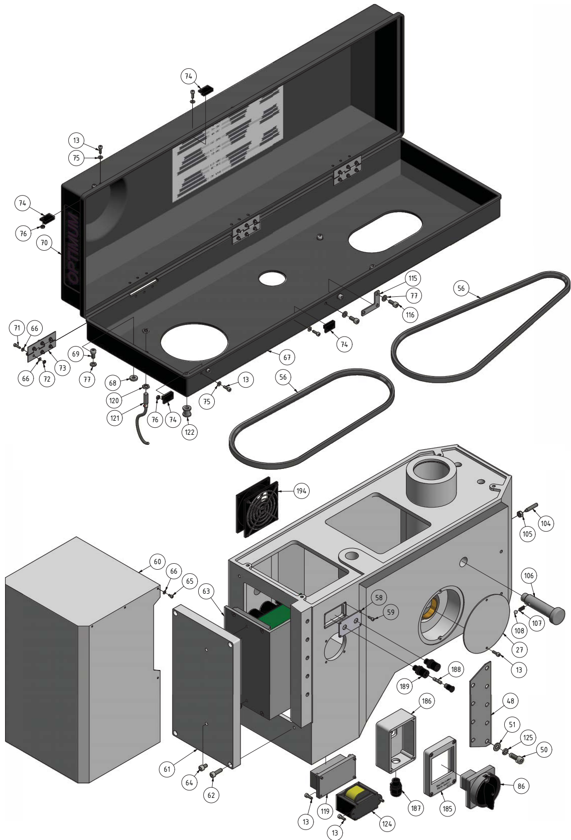
Abb. 1-16: Bohrkopf 5 von 5 - Drilling head 5 of 5
