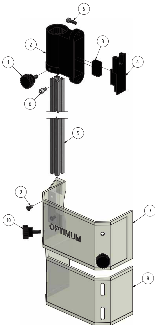
Img.1-6: Fräsfutterschutz - Milling chuck cover
