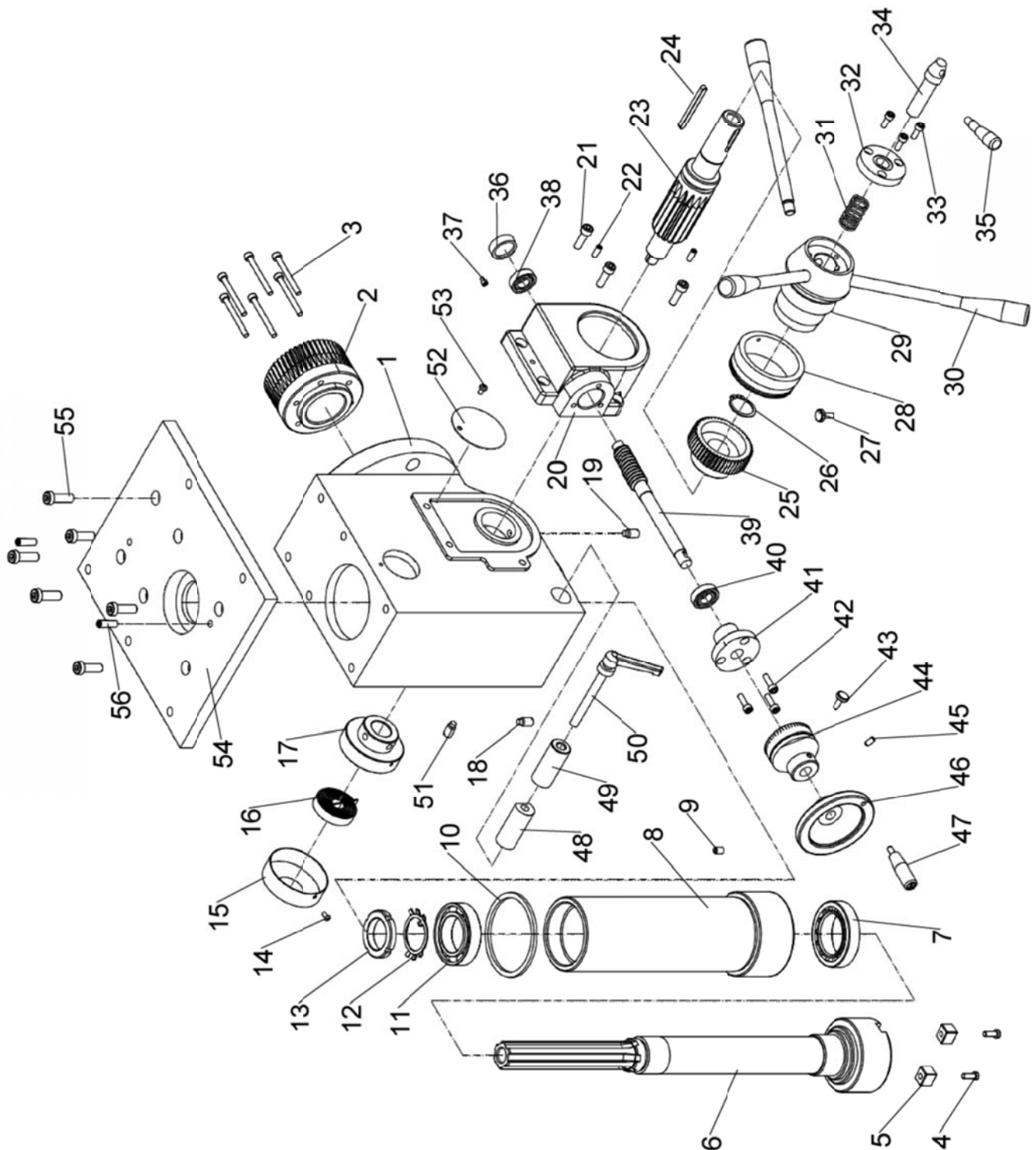
Abb.1-5: Universal Schwenkkopf - Universal swiveling head
