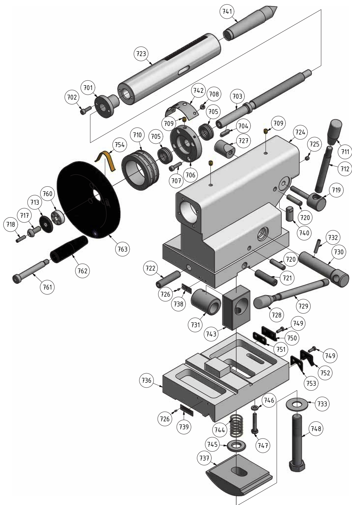
Img.1-22: Reitstock - Tailstock
