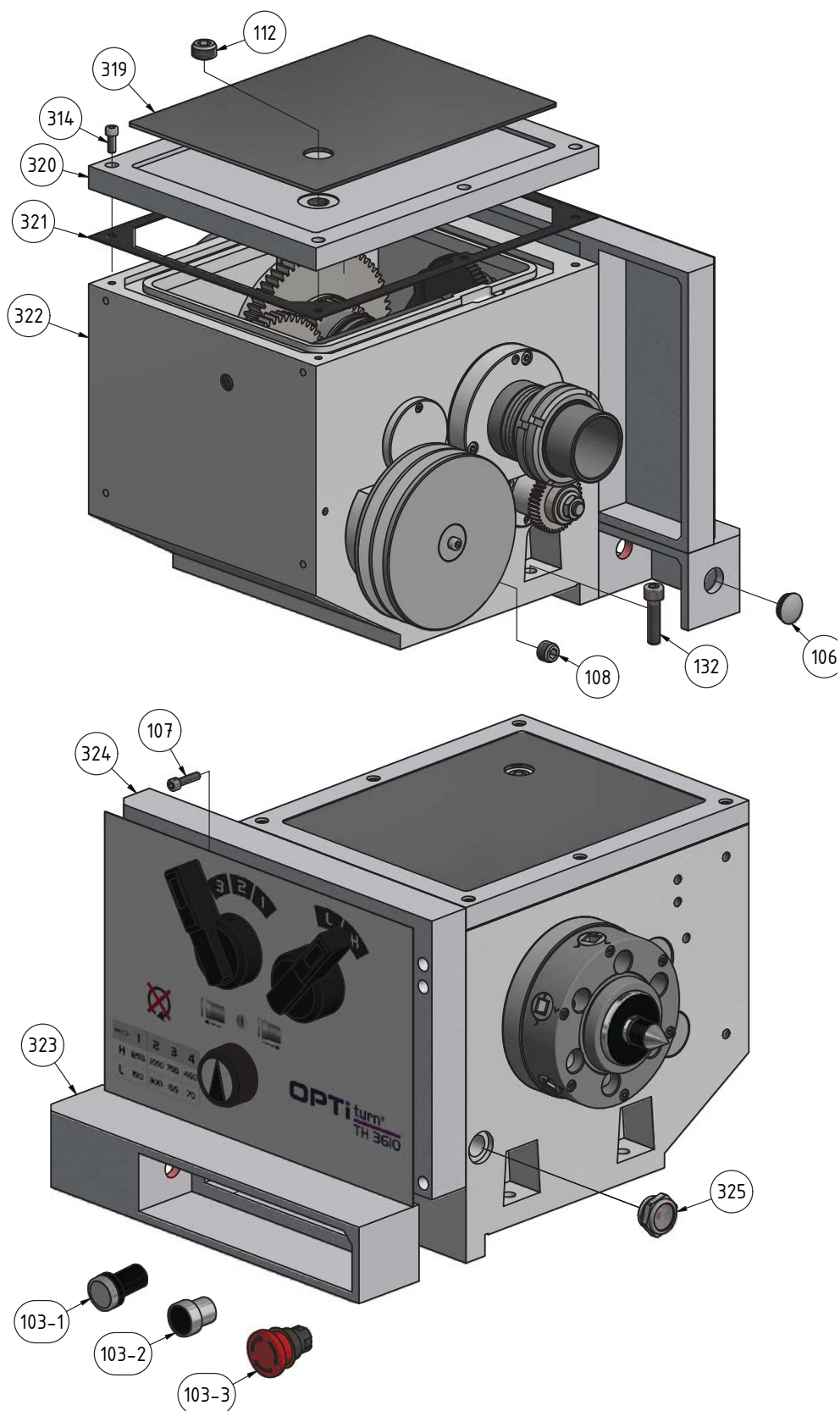
Img.1-4: Getriebe Spindelstock 1-6 - Headstock gear 1-6
